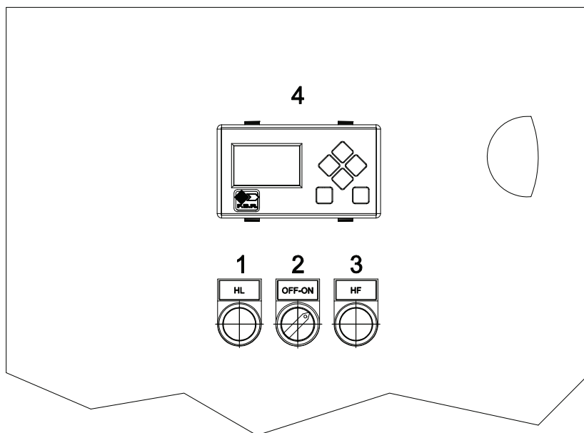
Fig. Burner control panel
