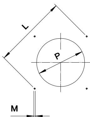
Fig. 4 Boiler plate
