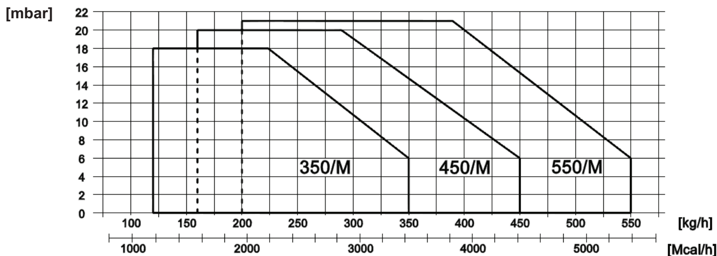
Fig. 2 X = Flow/Thermal power Y = Pressure in the combustion chamber
