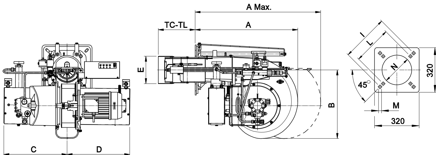
Fig. 2 Dimensions FNDP 100/2 - FNDP 125/2 - FNDP 150/2
